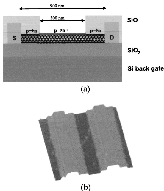
FIG. 1. (a) Device design, including the \text{SiO} passivation over the Ti/Au electrodes and neighboring area. The center of the device, which is left bare of \text{SiO} , is exposed to \text{NH}_3 or PEI. (b) Atomic force microscopy image of the SWNT contact passivated device after deposition of PEI. The image size is 2.75 \mu\text{m} .
