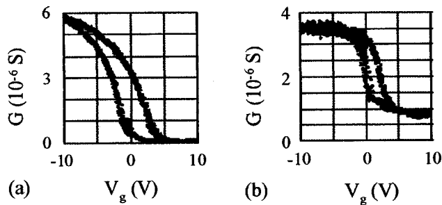
FIG. 2. Electrical properties of the SWNT devices at room temperature before and after passivation. Conductance vs gate-voltage G-V_g curve (100 mV bias). (a) non-passivated NT device and (b) SiO contact-passivated NT device.
