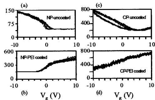
FIG. 4. The effect of PEI coating on transfer characteristics. (a) Nonpassivated NT device before coating; (b) nonpassivated NT device after coating; (c) contact-passivated NT device before coating; and (d) contact-passivated device after coating.
