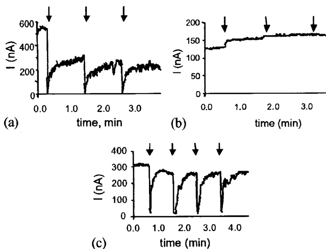
FIG. 3. Electrical response of SWNT device to gas. Current vs time (100 mV bias) recorded with short exposures to \text{NH}_3 with arrows indicating exposures. (a) Nonpassivated NT device with \text{NH}_3 ; (b) SiO fully passivated; (c) SiO contact-passivated. The metallic nanotube current has been subtracted from all three curves.
